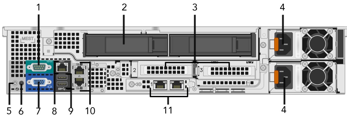
Figure 3. Rear view
