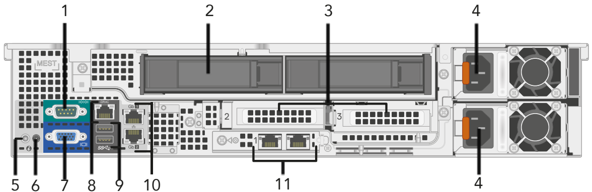
Figure 3. Rear view
